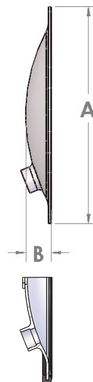
SECTION A-A (with Gasket Installed)
