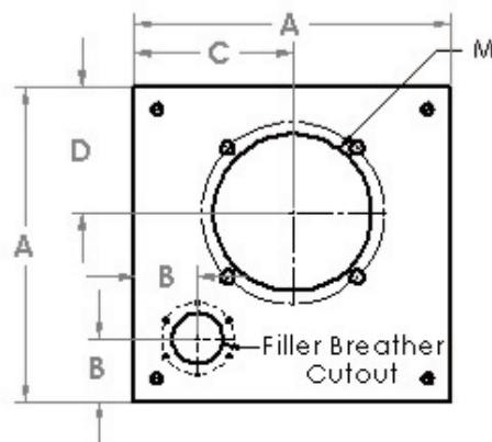
Cover w/Filler Breather and Pump/Motor Mount Cutout
