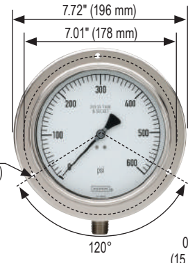
40-410/510 Front Flange
