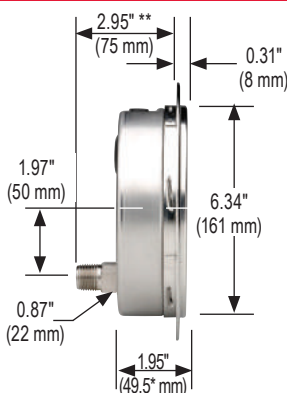
60-410/510 Front Flange
