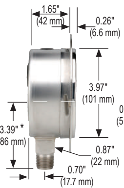
40-400/500 Front Flange
