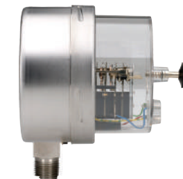
40-400 Series Gauge with Magnetic Spring Contact Switch
