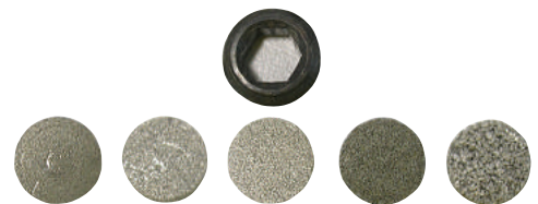
Sintered Snubbers Replacement Discs
