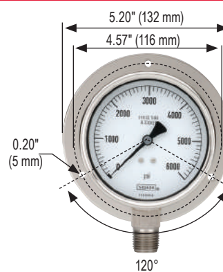
40-400/500 Rear Flange
