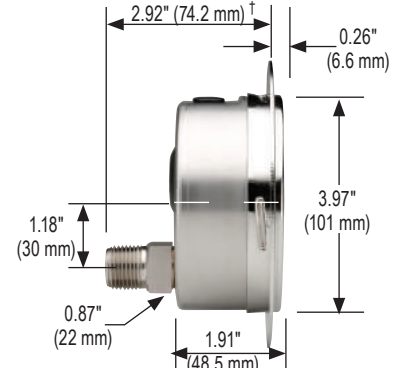
40-400/500 Rear Flange
