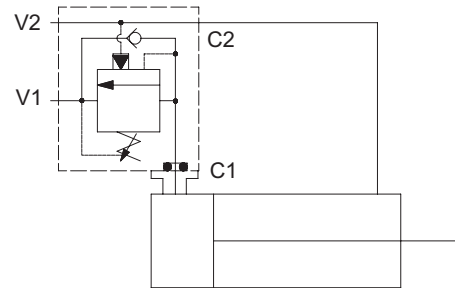
Single Counterbalance, Cap Mounted
