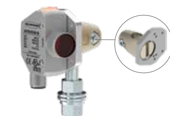
SMBQ4XFAM12 clamps directly onto industry standard bracket systems of 1/2" or 12 mm rods
