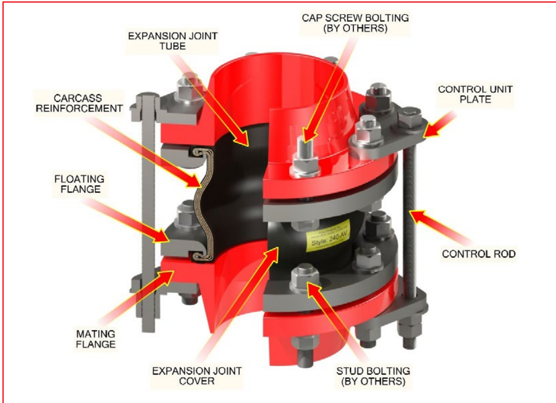
Shown as 240 Single Arch Design with Limit Rod (Figure 1)
