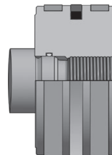
Schrader Bellows KP Filled PTFE Piston Seal
