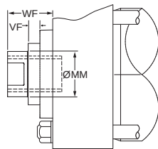
Style 9B – Short Female
