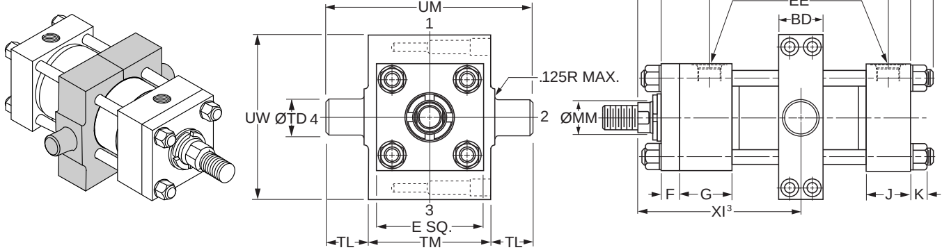
Style DD – Dimensional and Mounting Data
