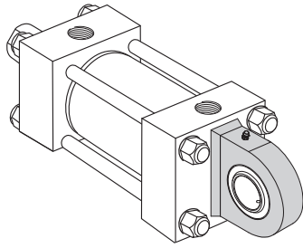
Style SE — Dimensional and Mounting Data
