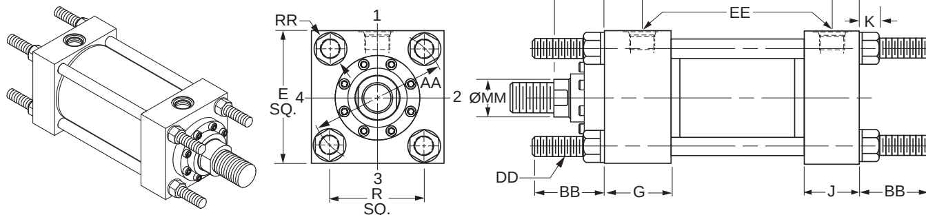
Style TD – Dimensional and Mounting Data
