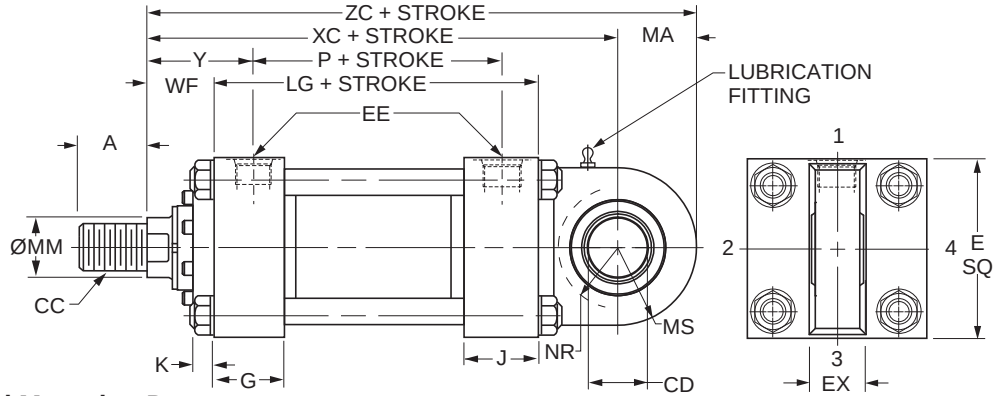
Style SE — Dimensional and Mounting Data
