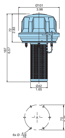
Six-Hole Option
