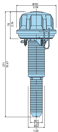
Telescopic Strainer
