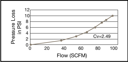
Flow Curve - Pressure Loss
