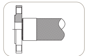
8K - Raised Face, 150lb Fixed Slip-on Flange
