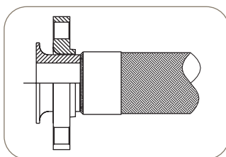
4K - Schedule 40 Type A Stub, 150lb Lap Joint (Floating) Flange
