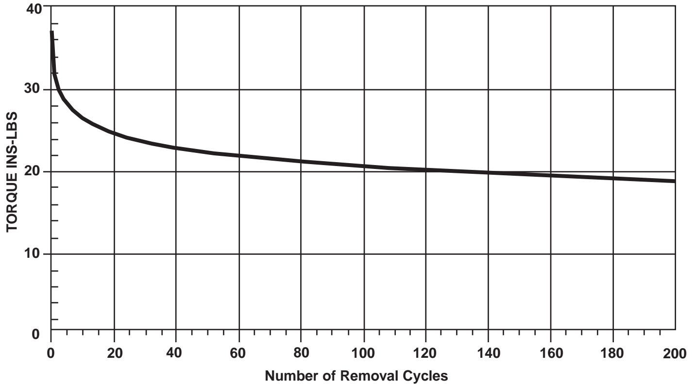
Removal Torque for -10 Titanium, Beam Seal
