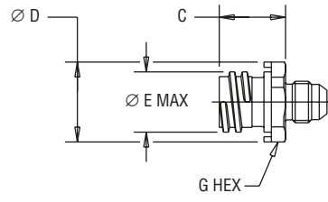
NIPPLE
