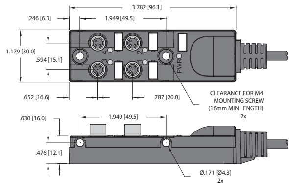
4-Port Threaded with Integral Home Run Cable
