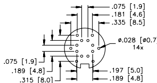
7-Pin PCB Layout
